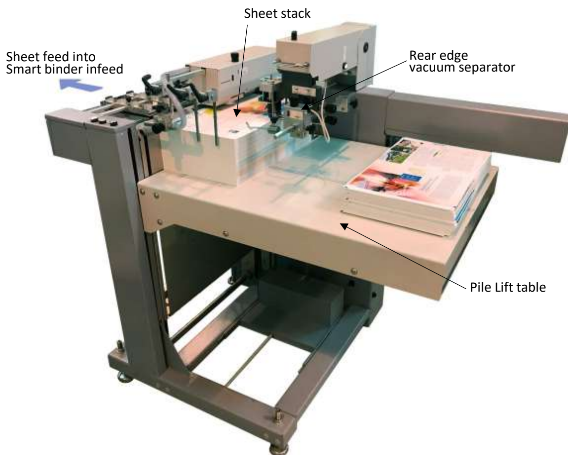
Sheet pile feeder SB-095
