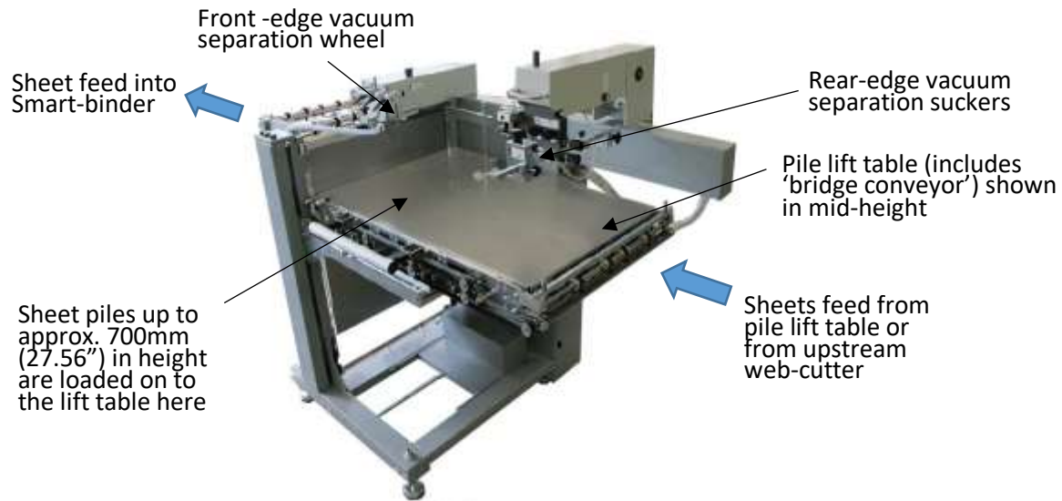
Sheet pile feeder SB-097
