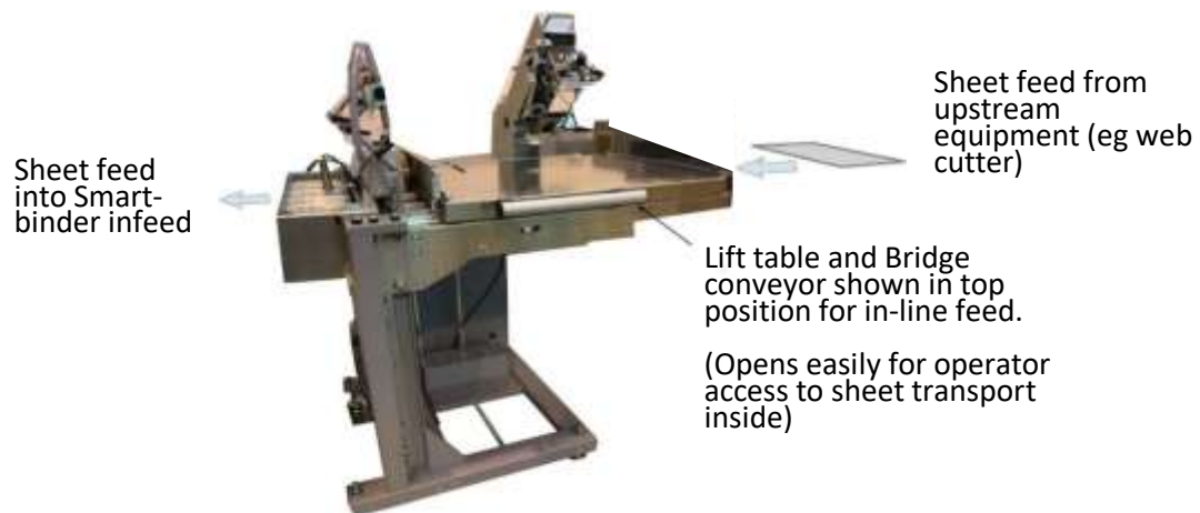
SB-097 in its upper position, to run in-line
